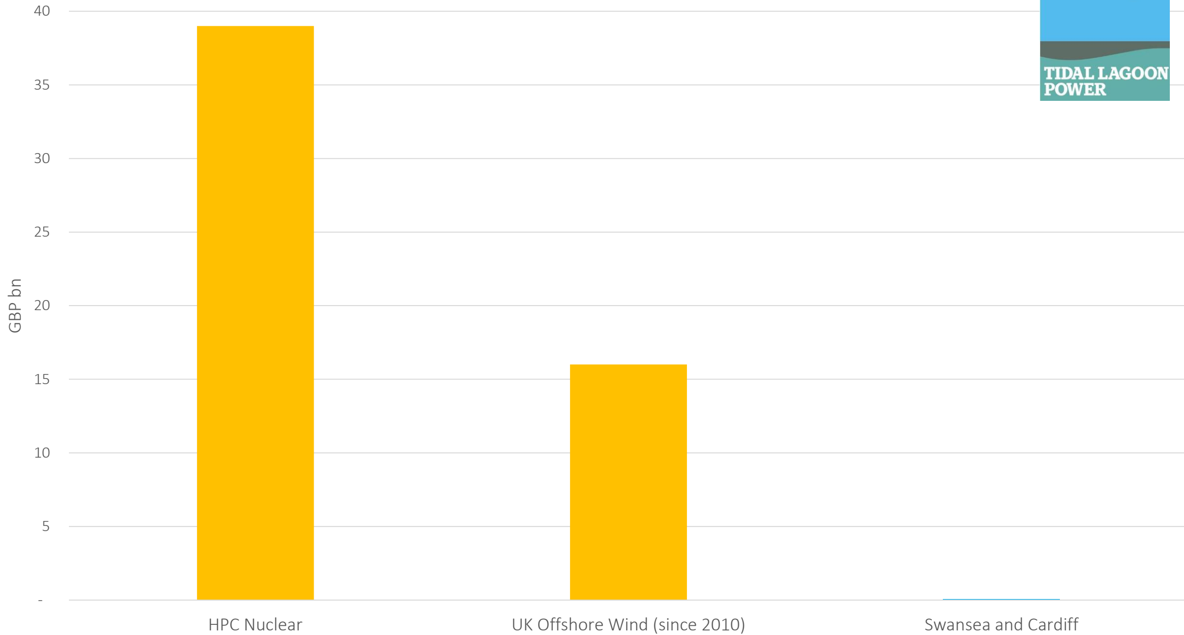
Comparison of subsidy required/received between Hinkley Point C, offshore wind and Swansea and Cardiff Lagoons
